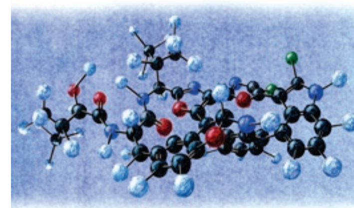
The diazomamide A molecule: black = carbon, white = hydrogen, red = oxygen, blue = nitrogen and green = chlorine
